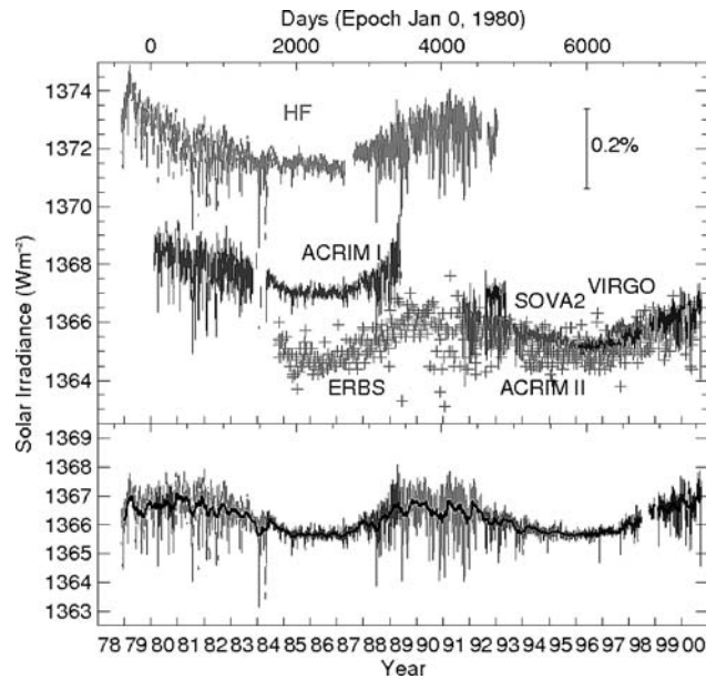
Figure 1. The various total irradiance time series are presented in the upper panel , the composite total solar irradiance is shown on the lower panel (updated from Fröhlich, 2000; courtesy J. Pap, 2003).
