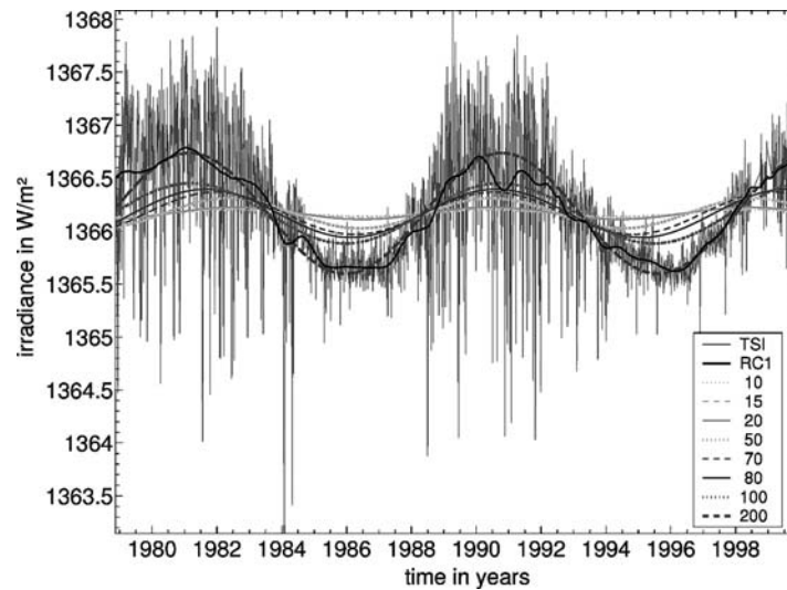
Figure 2. Variation of solar luminosity associated with a temporal sinusoidal change of the solar radius. Dashed lines, solid gray line or dot line represent the Total Solar Irradiance (TSI) and the plain black curve its RC1 component (trend, see text). The successive sinusoidal curves show the irradiance variations computed through successive values of dR : the trend is rather well explained by a 200-mas radius amplitude variation, but such a large value is excluded. However, up to a 10-mas radius amplitude variation still explains part of the trend.
